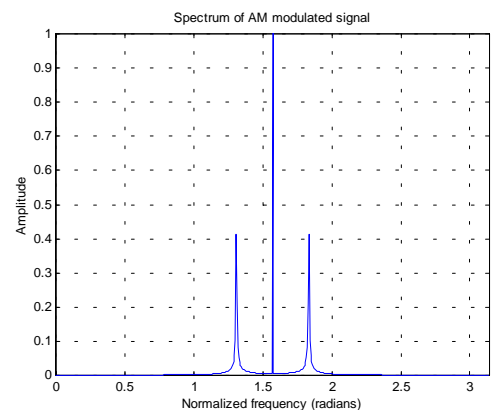
Figure 3 Amplitude modulation, f_c is \pi/2 and modulating signal contains frequency of \pi/12 .
