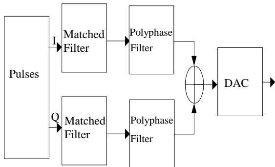
Figure 4 Digital modulator with interpolation
