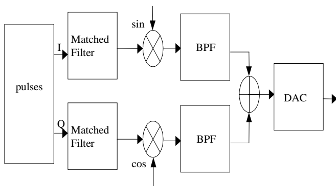
Figure 1 Conventional heterodyning digital modulator
