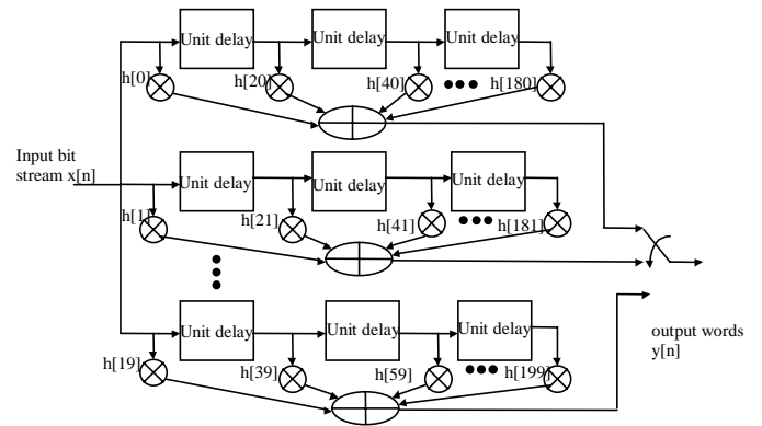
Figure 5 Polyphase implementation of 200 taps FIR filter
