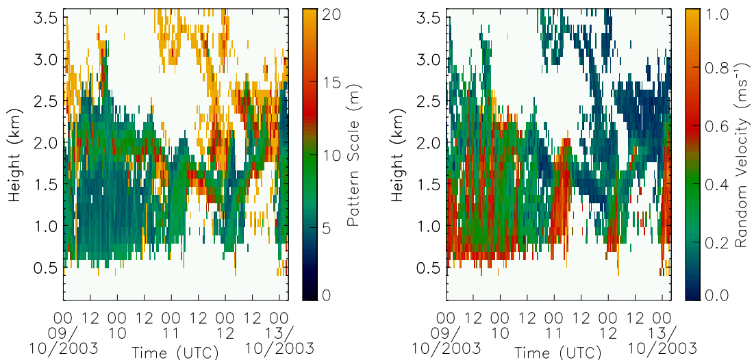
Figure 6: Pattern scale (left) and random velocity ( V_{rms} ) (right) obtained for the Mini-BLR, 9th to 13th October 2003 (30 min. averages).
