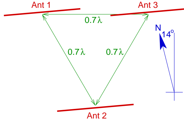
Figure 1: Layout of Mini-BLR at Buckland Park during October 2003 trials.
